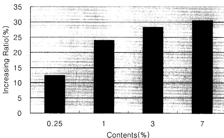
Figure 6. The increasing ratio of emissivity of the O/W emulsion containing the jade powder. The y-axis is the increasing ratio (percentile) and the x-axis is the contents of the jade powder.
