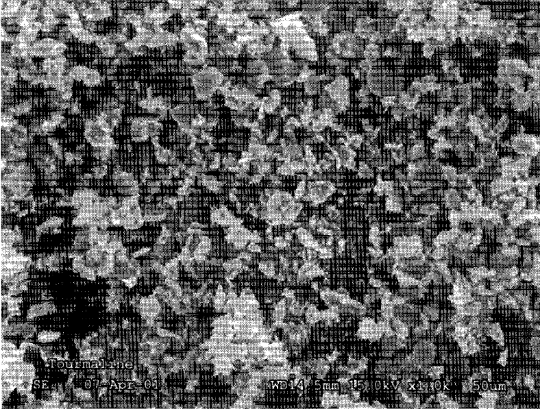
Figure 1. SEM observation of tourmaline powders ( \times 1000 ). The crystal structure used was a mixture of a round-type crystal and a plane-type crystal, and had a mean diameter of 10 micrometers.
