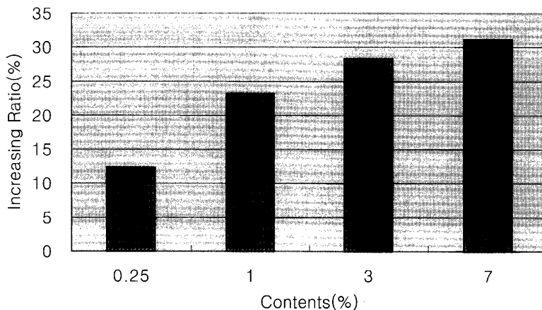
Figure 5. The increasing ratio of emissivity of the O/W emulsion containing the tourmaline powder. The y-axis is the increasing ratio (percentile) and the x-axis is the contents of the tourmaline powder.
