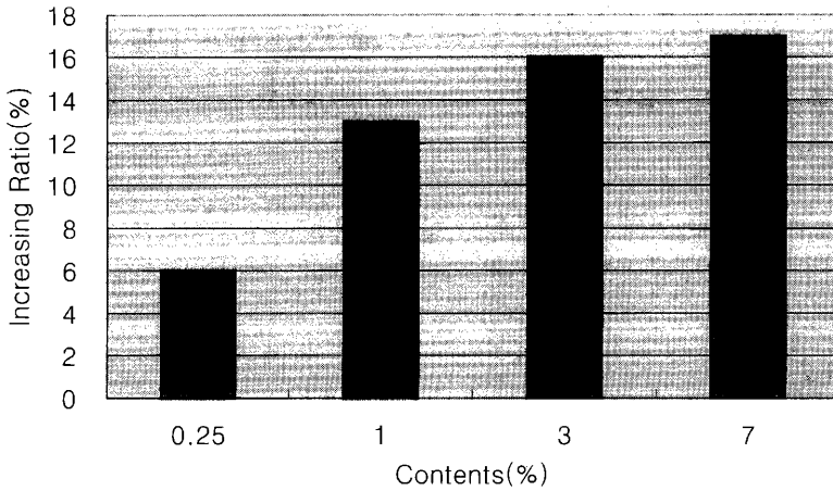
Figure 3. The increasing ratio of radiation energy ( \text{W}/\text{m}^2 ) of the O/W emulsion containing the tourmaline powder. The y-axis is the increasing ratio (percentile) and the x-axis is the contents of the tourmaline powder.
